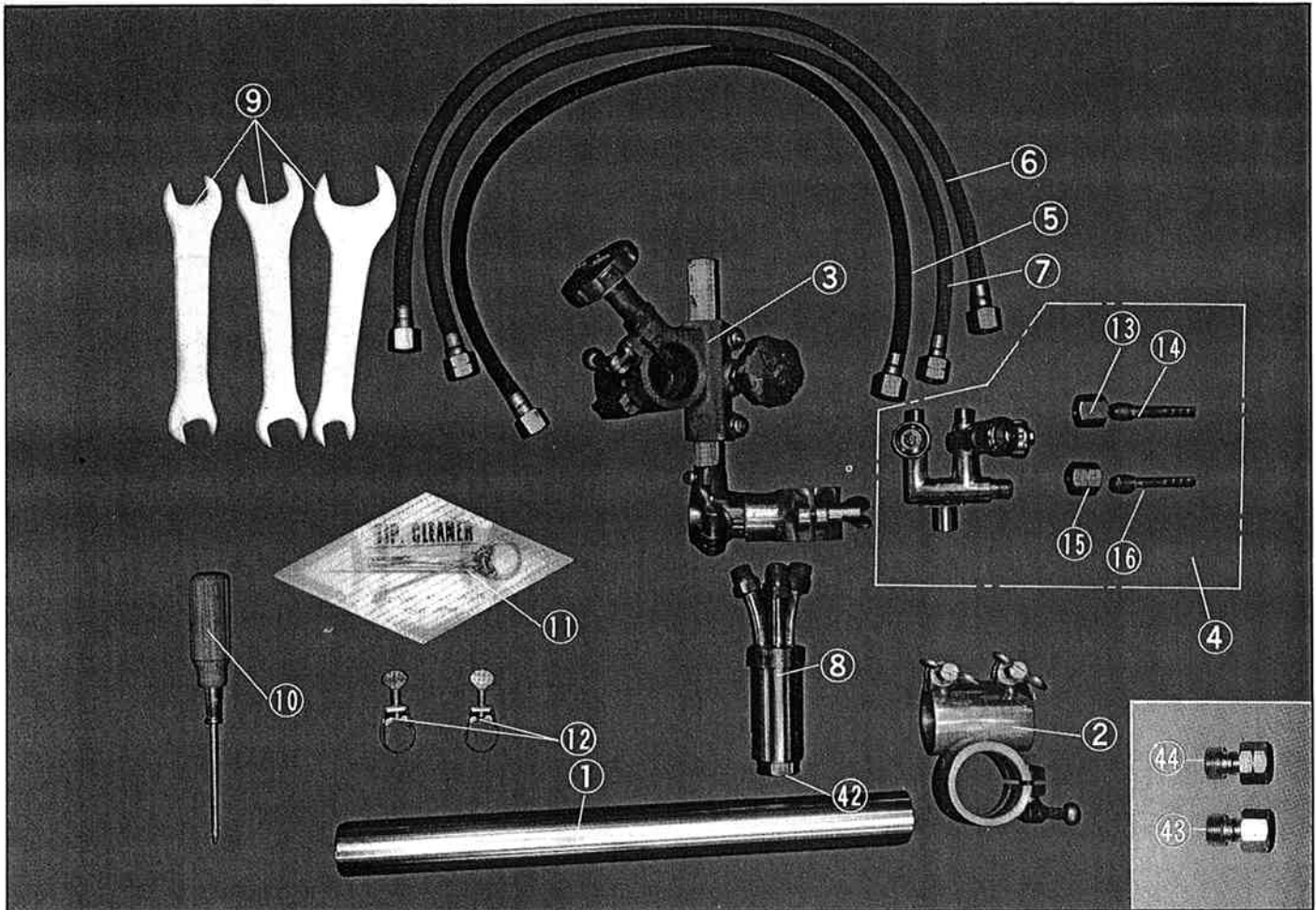
PARTS LIST
