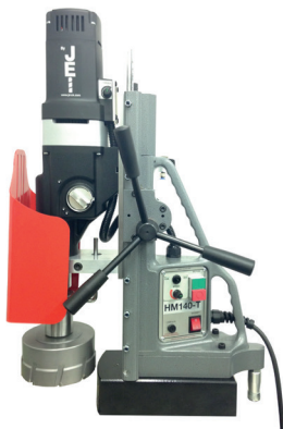
50mm 4MT twist drill capacity
